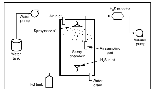
Figure 2. Schematic diagram of laboratory set-up used to determine the effect of water-based spray on H 2 S levels in the chamber.
