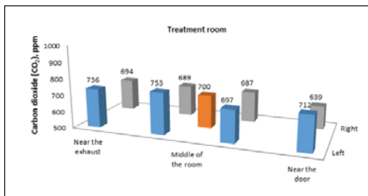
Figure 2. Average CO 2 concentrations measured at the animal-occupied zones in the Control and Treatment rooms in winter trials
